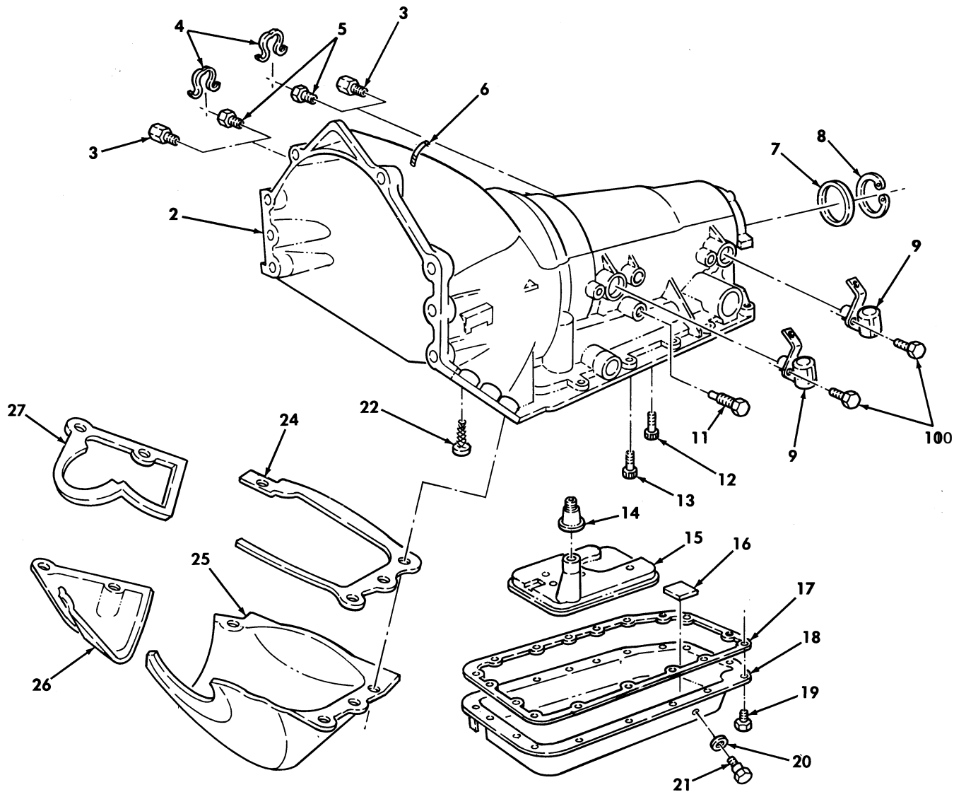
Figure 105. Transmission Assembly.
