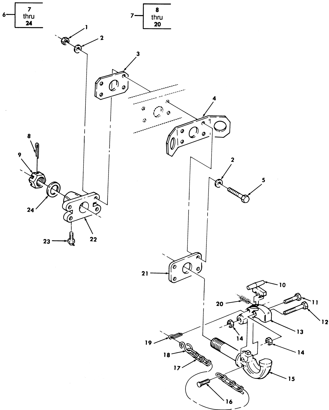
Figure 191. Towing Pintle Assembly.
