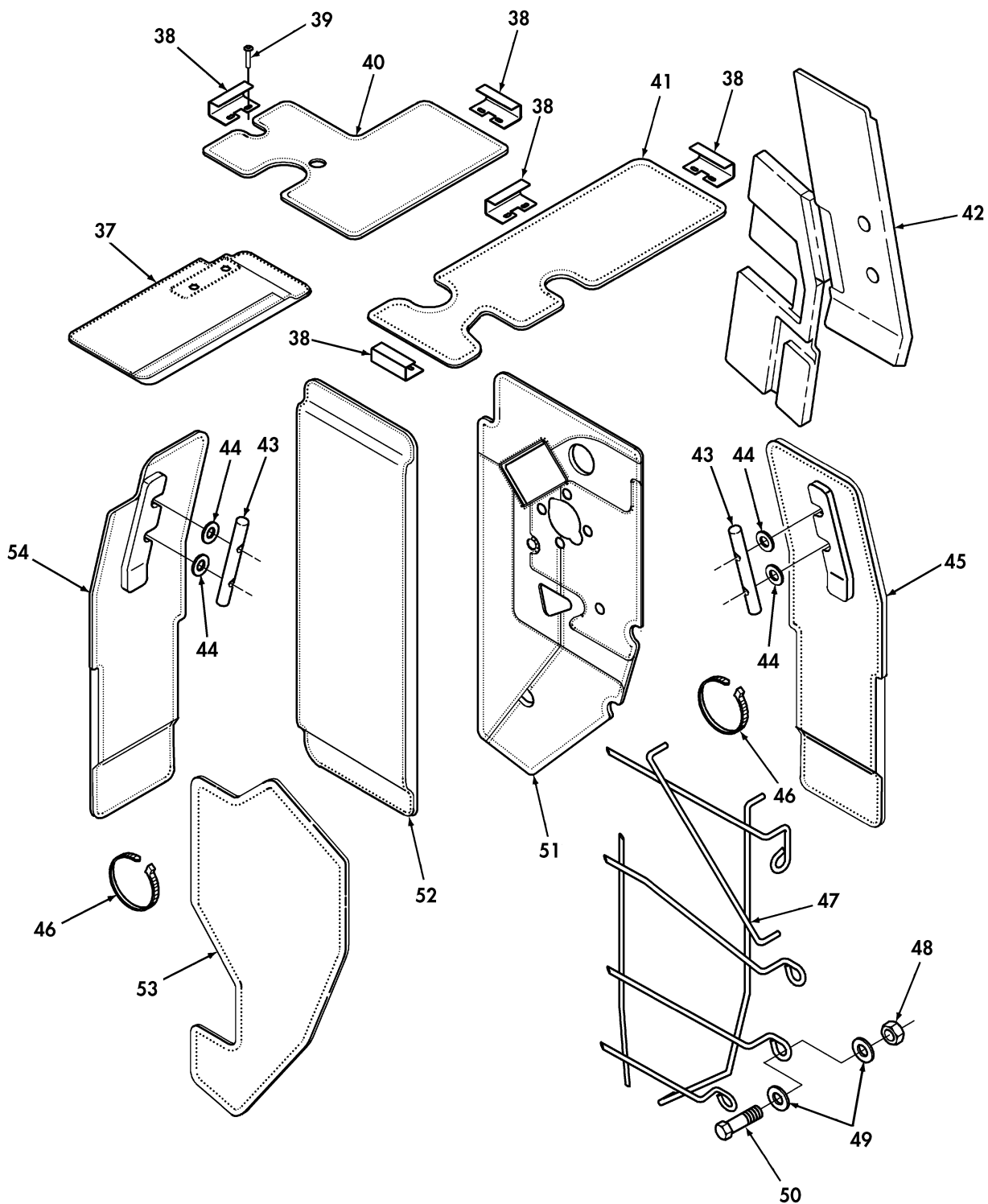
Figure 227. Interior Tunnel, Cowl, Floor Insulation, Mounting Components (Foam), and Exterior Insulation (Sheet 2 of 2).
