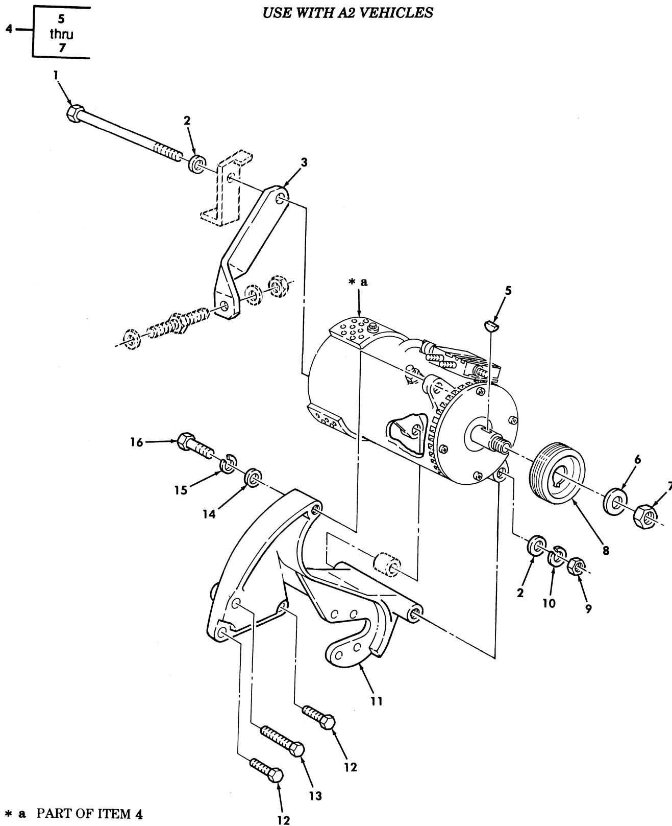
Figure 36. 100 AMP Alternator (NIEHOFF) and Mounting Hardware.
