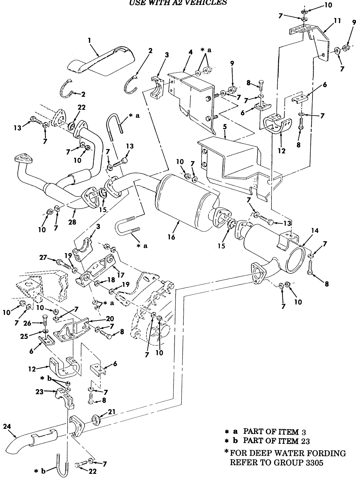
Figure 24. Muffer, Exhaust Pipes, and Related Parts.
