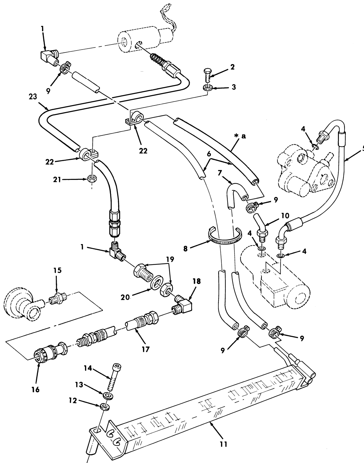
Figure 178. Power Steering Oil Cooler, Hydro-Booster, and Fan Clutch Hydraulic Lines and Fittings.
