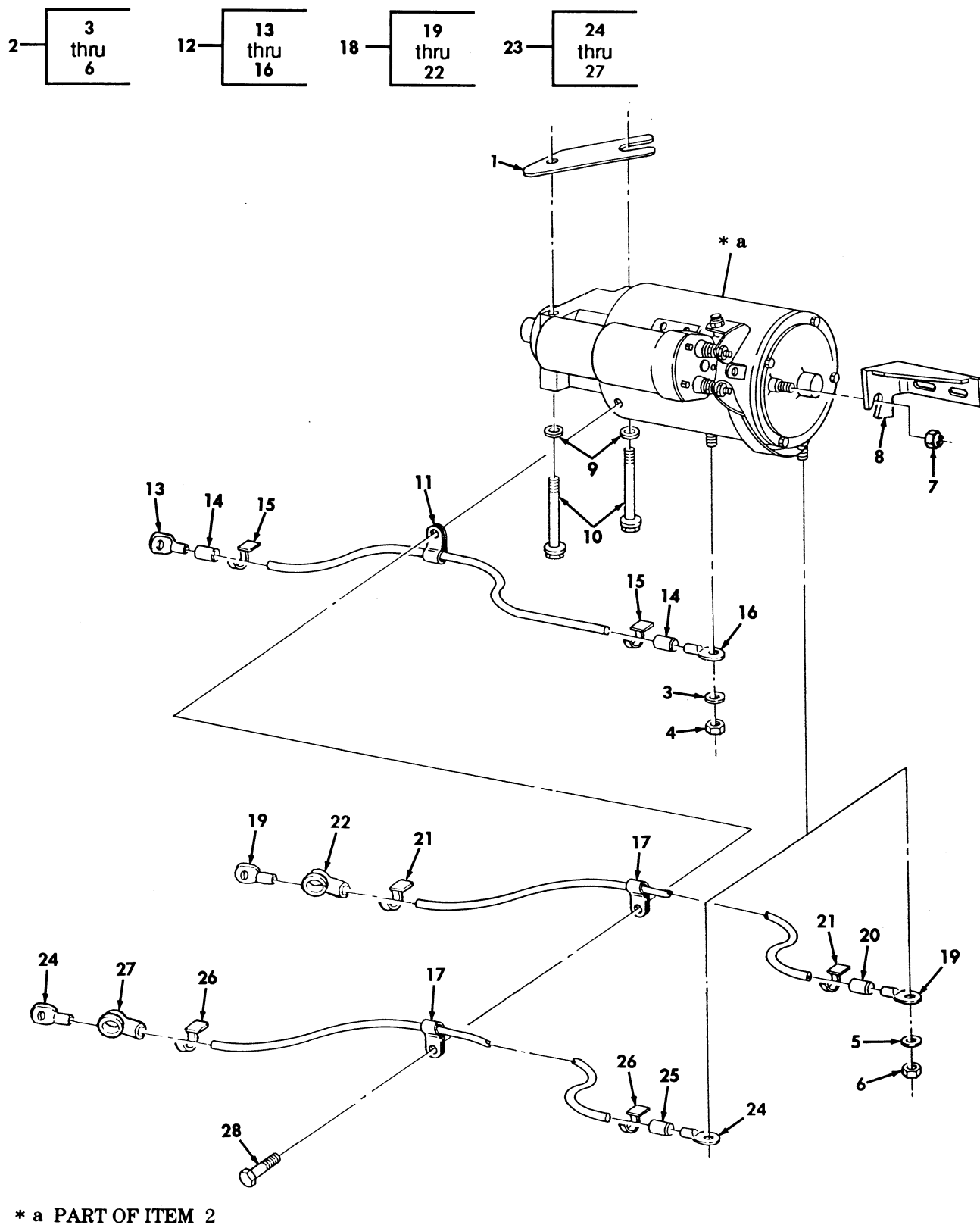
Figure 44. Starter Motor, Cable Assemblies, and Mounting Hardware.
