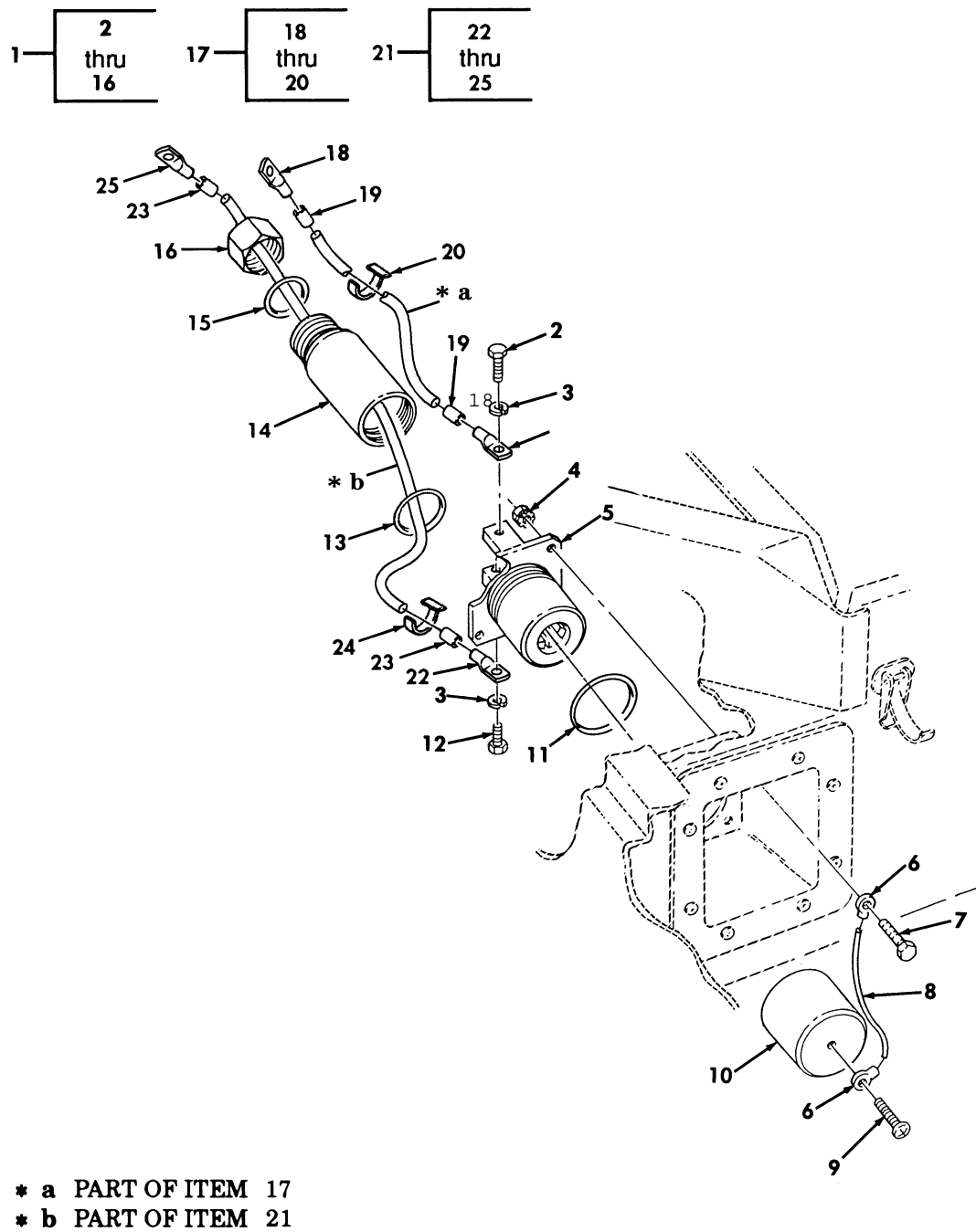
Figure 73. Slave Receptacle and Cable Assemblies.
