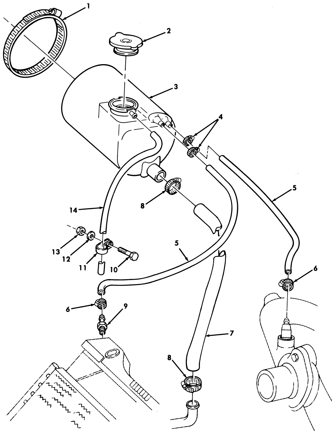
Figure 27. Surge Tank and Related Parts.
