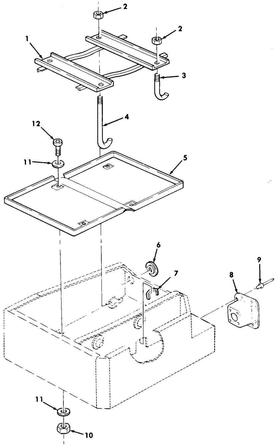
Figure 71. Battery Mounting Components and Related Parts.
