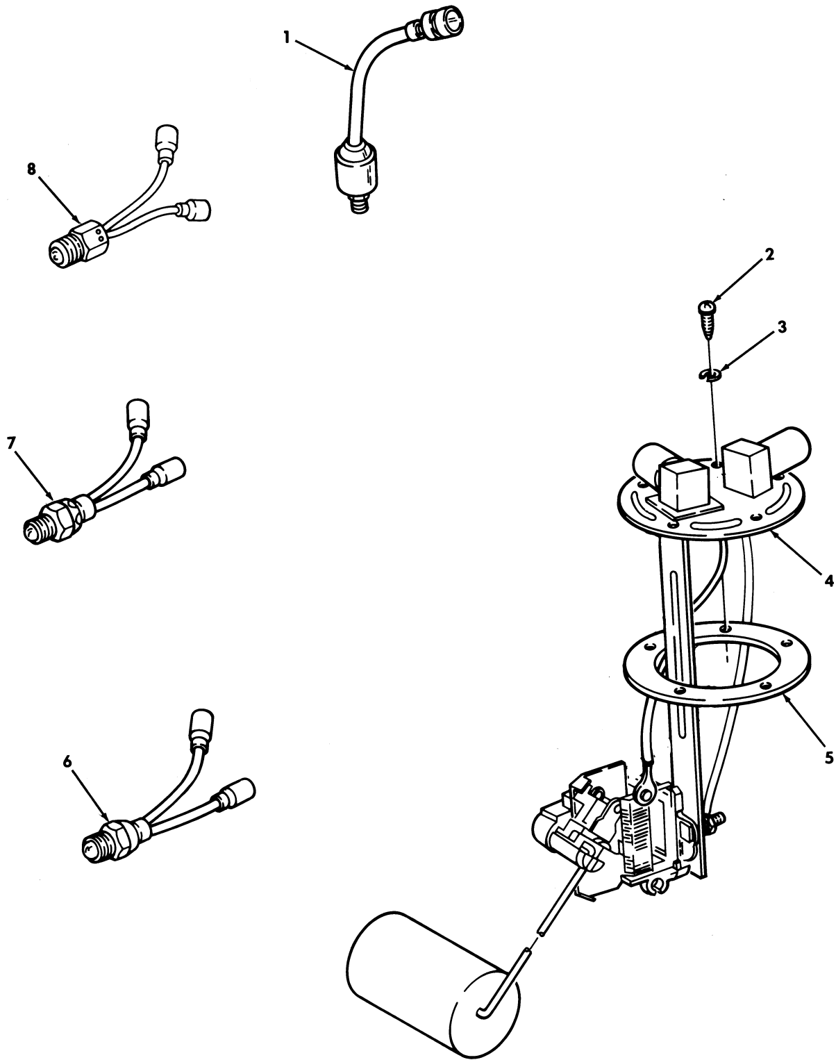
Figure 67. Fuel Pressure Transducer, Fuel Level Transmitter, Parking Brake, Backup Light Switches, and Transfer Indicator Switch.
