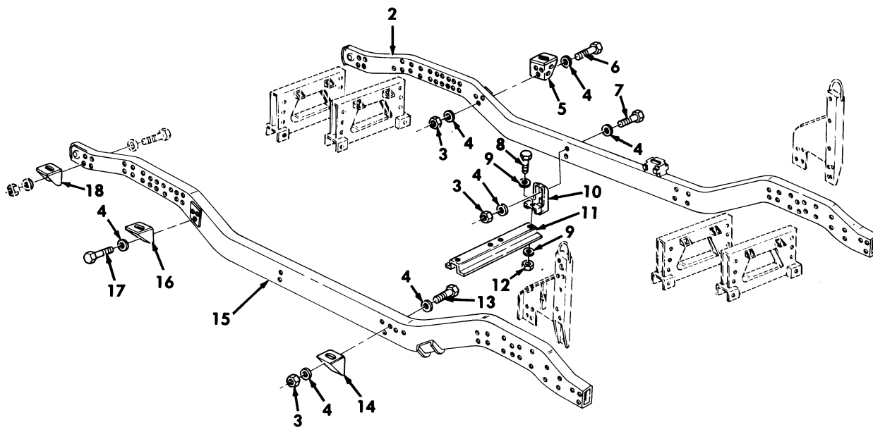
Figure 179. Frame Assembly, Body Mount Brackets, and Transmission Crossmember.
