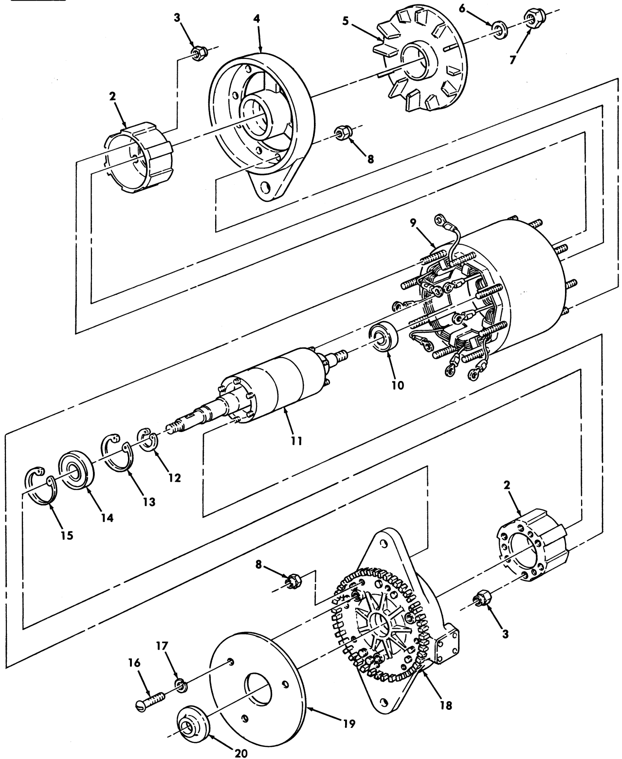
Figure 40. 200 AMP Alternator, M996, M996A1, M997, M997A1, M997A2, M1097, M1097A1, M1097A2, and M1123 (NIEHOFF) (Sheet 1 of 2).
